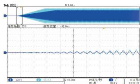
零压启动转CC
