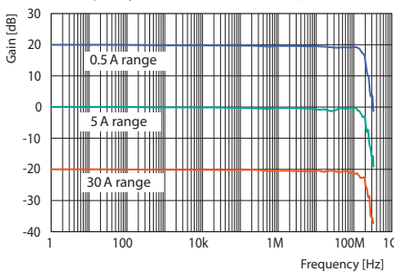
Frequency characteristics: CT6711 (Typical)
