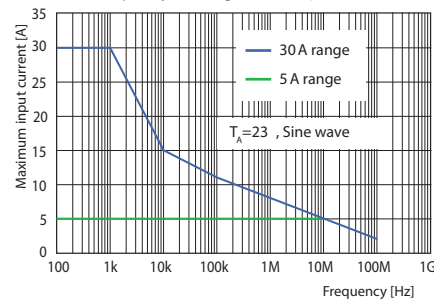
Frequency derating: CT6711 (Typical)
