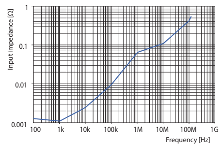
Input impedance: CT6711 (Typical)
